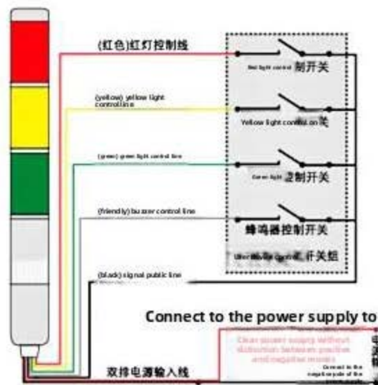
220v wiring diagram
